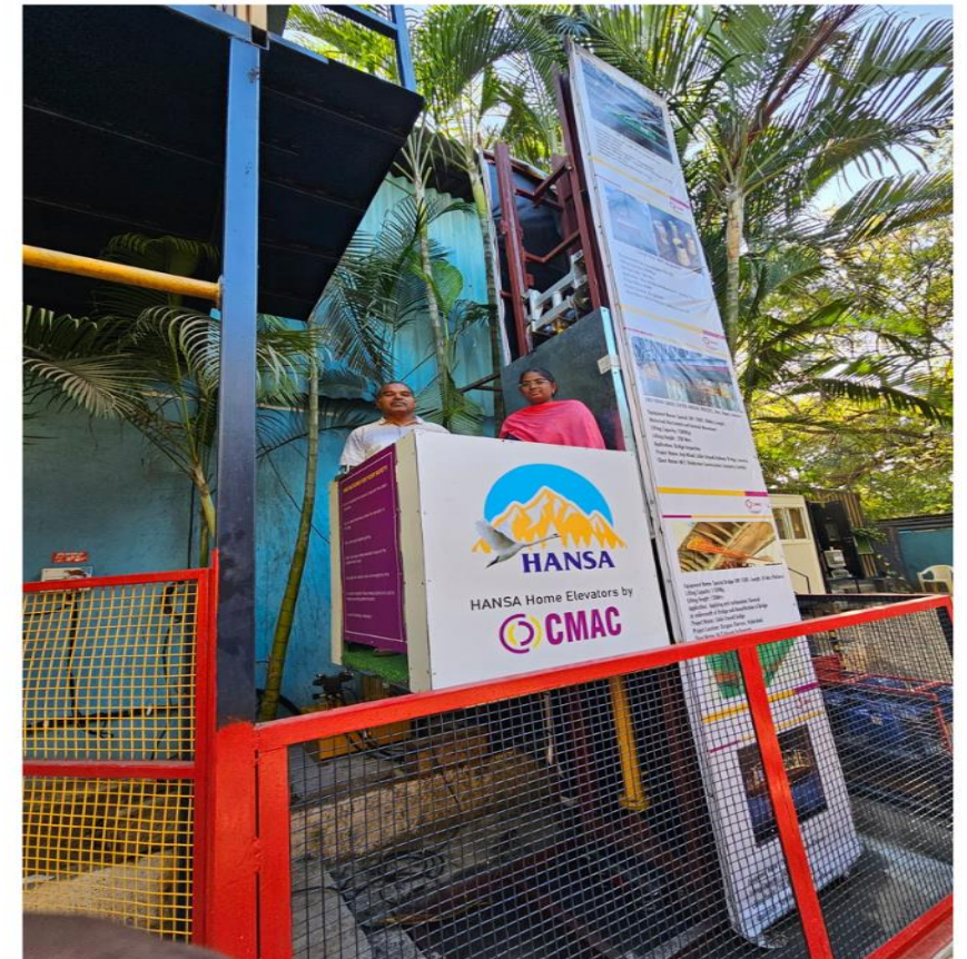
Hydraulic Lift with ACP Sheet Encloser
